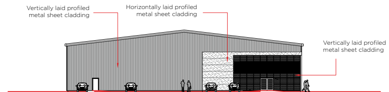
UNIT A SOUTH ELEVATION
