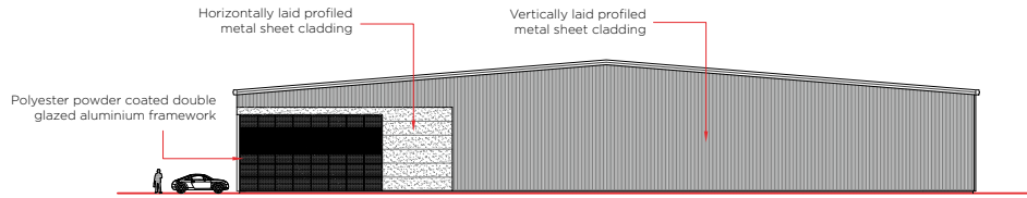
UNIT B EAST ELEVATION
