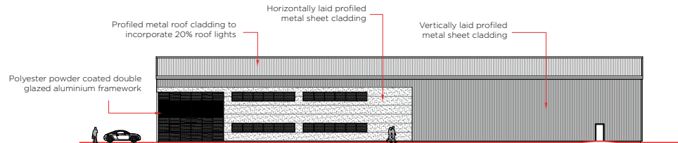
UNIT A EAST ELEVATION
